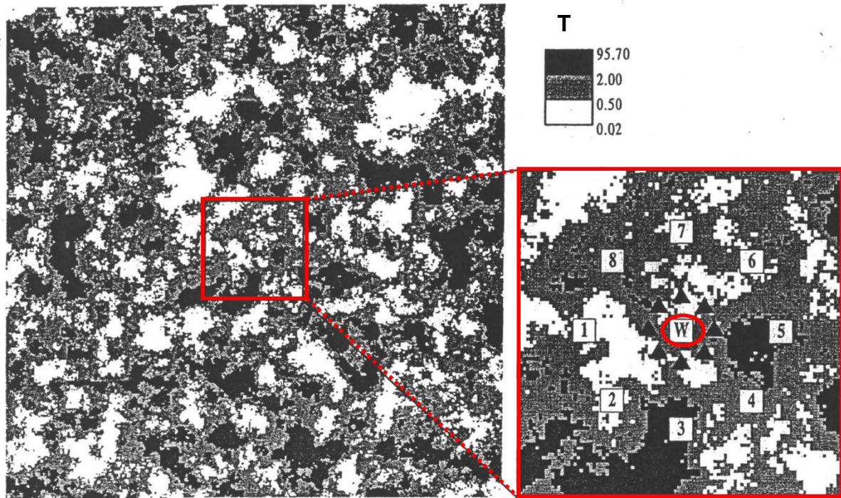
Figure 6. Random transmissivity field for \sigma^2 = 4.0 Adapted from Meier and others (1998; Figure 8)
