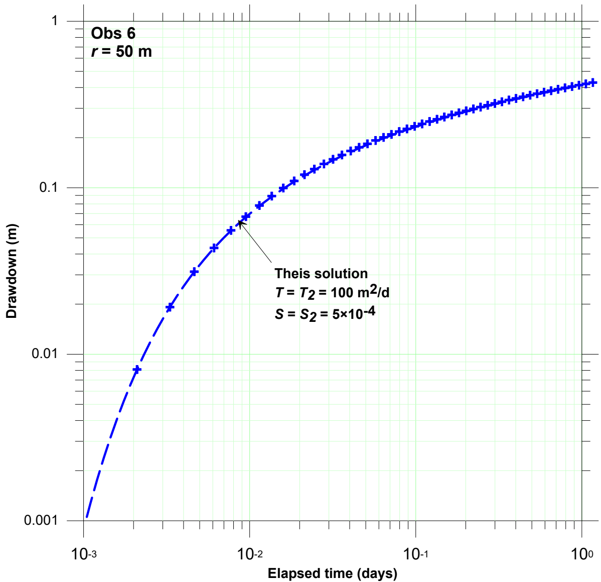
Figure 29. Theis analysis for observation well #6 ( r = 50 m)
