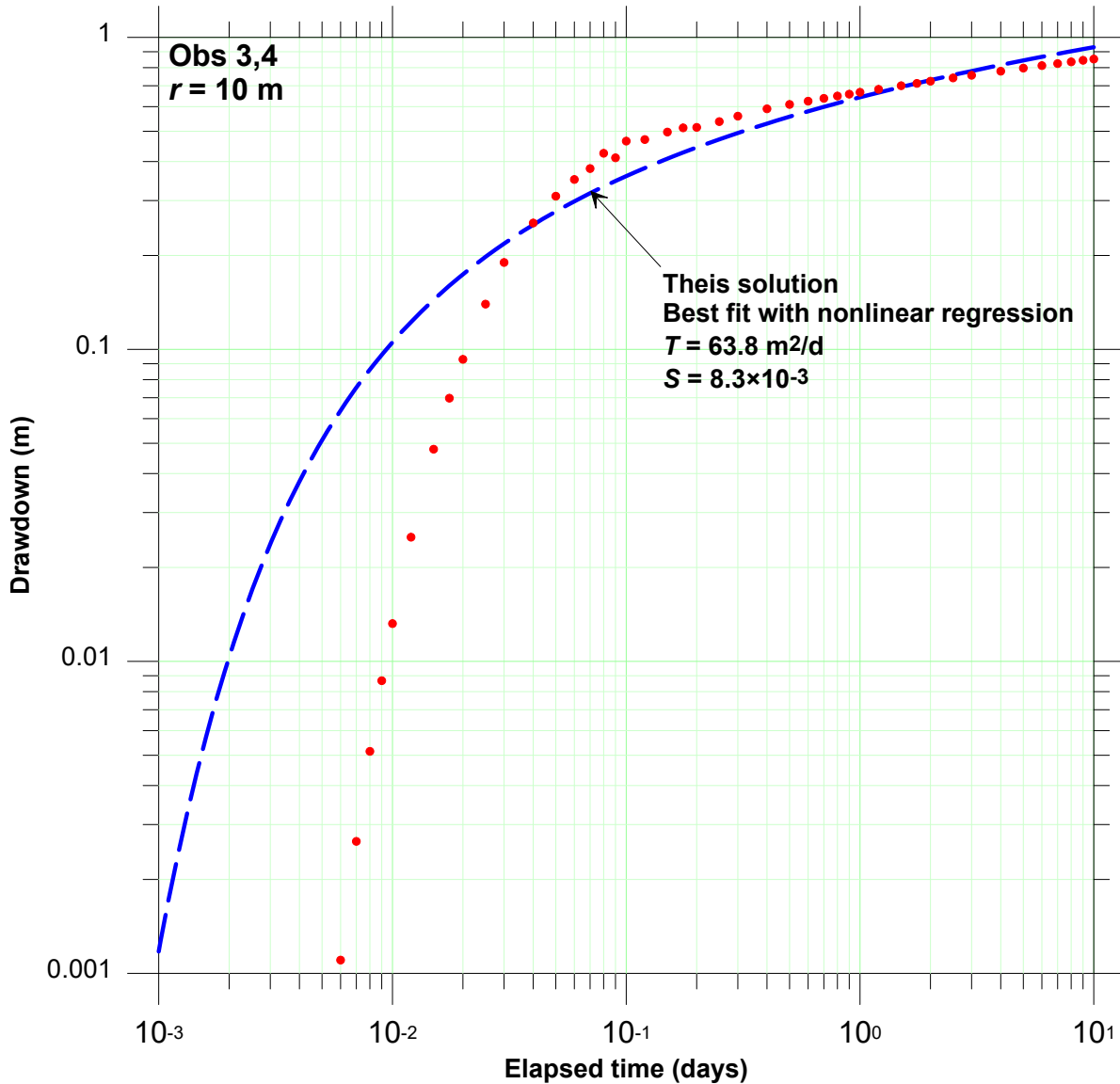
Figure 19. Match of the Theis solution to the drawdowns at observation wells at r = 10 \text{ m}
